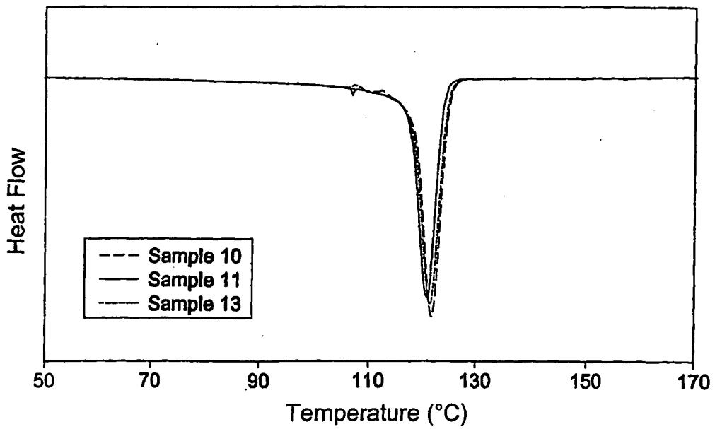
Fig. 8 DSC Crystallization of Plasticized Propylene Random Copolymers
